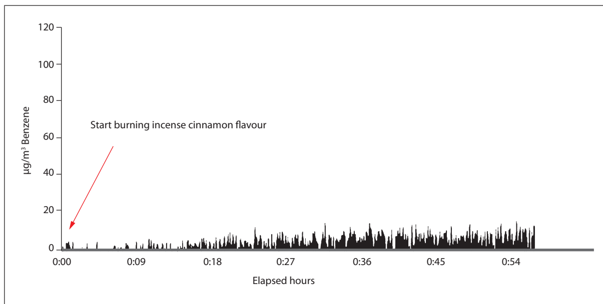
Figure 3 Time trend of the benzene concentration produced by burning cinnamon flavor incense.
