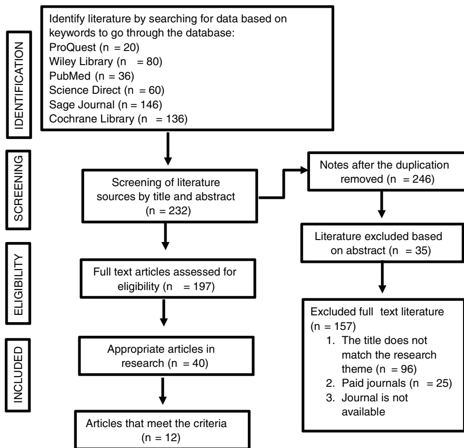
Figure 1. PRISMA flowchart.
