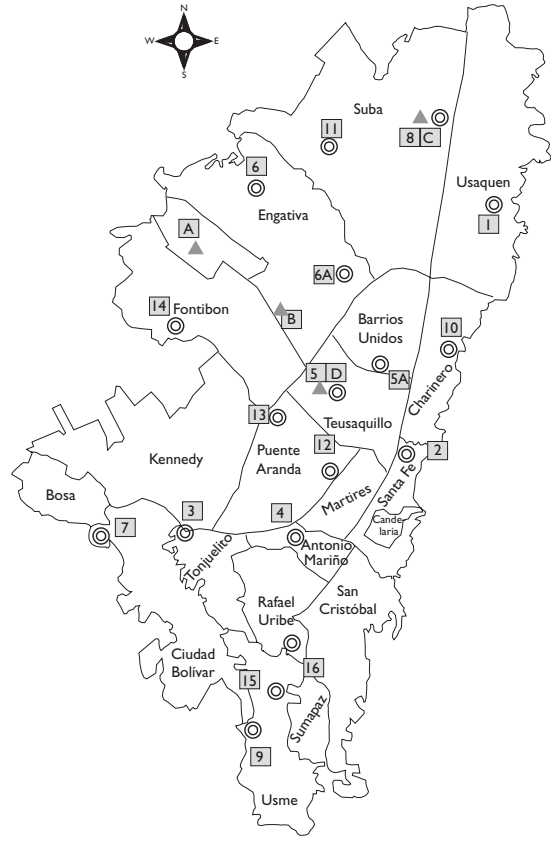
FIGURE 1. GEOGRAPHIC DISTRIBUTION OF AIR QUALITY MONITORING NETWORK STATIONS (RM CAB) AND THE INSTITUTE OF HYDROLOGY, METEOROLOGY AND ENVIRONMENTAL STUDIES (IDEAM) METEOROLOGICAL STATIONS. APRIL 1, 1998 TO DECEMBER 31, 2006, BOGOTA, DC.
